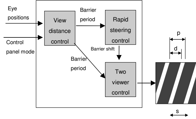
Figure 6: Controller block diagram illustrates three main functions: view distance, rapid steering, and 2-viewer control.
