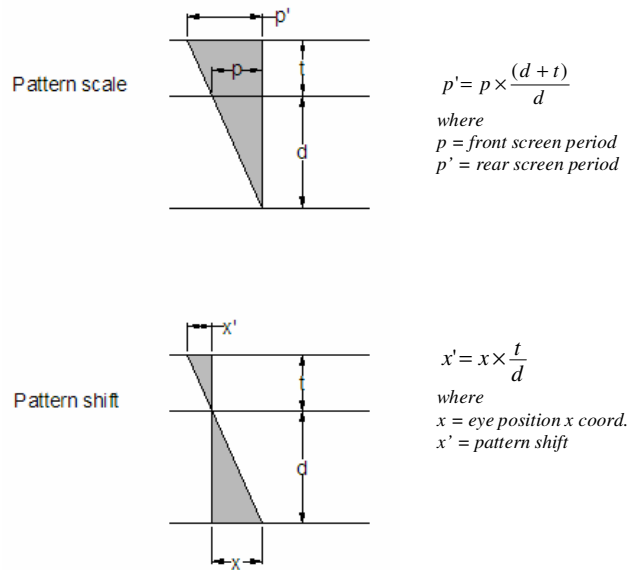
Figure 4: The barrier period and position between front and rear screens are related by a scale and shift operation.
