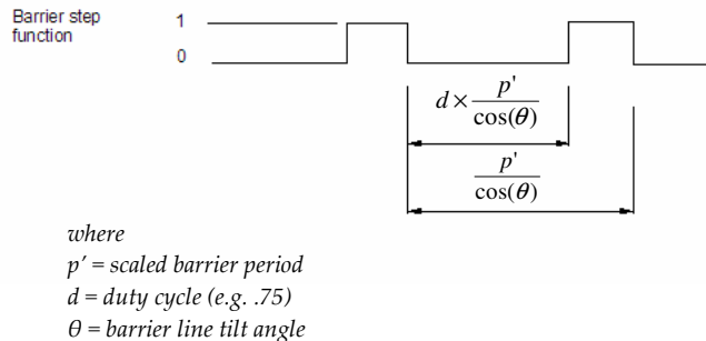
Figure 5: The barrier step function is shown.
