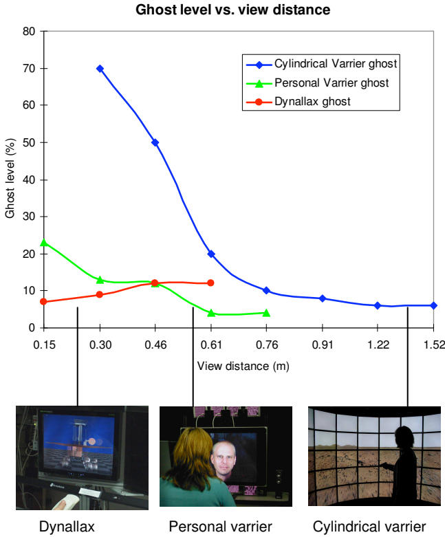
Figure 13: Ghost level vs. view distance is plotted for Dynallax and two Varrier implementations.
