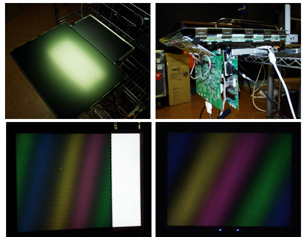
Figure 16. Photographs of the custom display are shown in the top row. Results with the custom display in the lower left and the PureDepth display in the lower right are comparable and encouraging.
