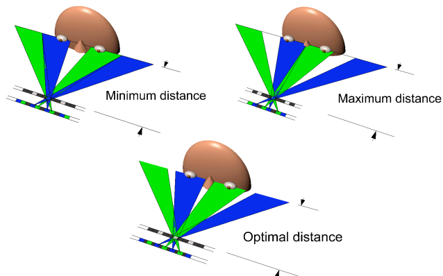
Figure 7: Spacing of channels in a static barrier system varies with view distance.
