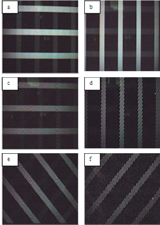
Figure 14: Left-eye and right-eye views under single-viewer and two-viewer modes are captured by cameras. a and b: left and right eye of single viewer mode; c and d: left and right eye of first viewer under two-viewer mode; e and f: left and right eye of second viewer under two-viewer mode. Different orientation white bars are rendered for the various channels, and the dim traces of opposite orientations are the ghost level of the system.
