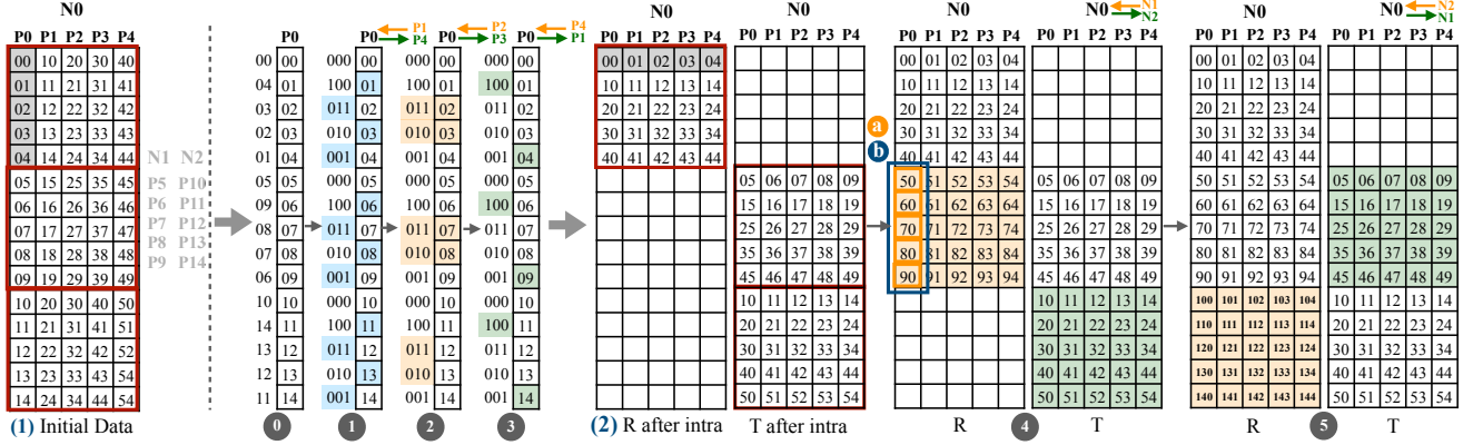
Figure 4: An example of ParLinNa when P = 15 , N = 3 , r = 2 and Q = 5 . (1) depicts the initial state in send buffer for all processes within node N_0 . Each process logically has Q data-blocks in every N group (separated by red boxes). ① shows the rotation index array for P_0 based on the group rank ID ( g = p \% Q ). ② ③ illustrate the three intra-node communication steps, where the sent data-blocks are colored. (2) presents the data status in receive ( R ) and temporary ( T ) buffers after the intra-node communication, where R holds the data-blocks destined the processes within N_0 . ④ ⑤ depict two steps for inter-node communication. (a) and (b) are two communication patterns (matching Figure 5). Finally, each process receives the required data-blocks in R .
