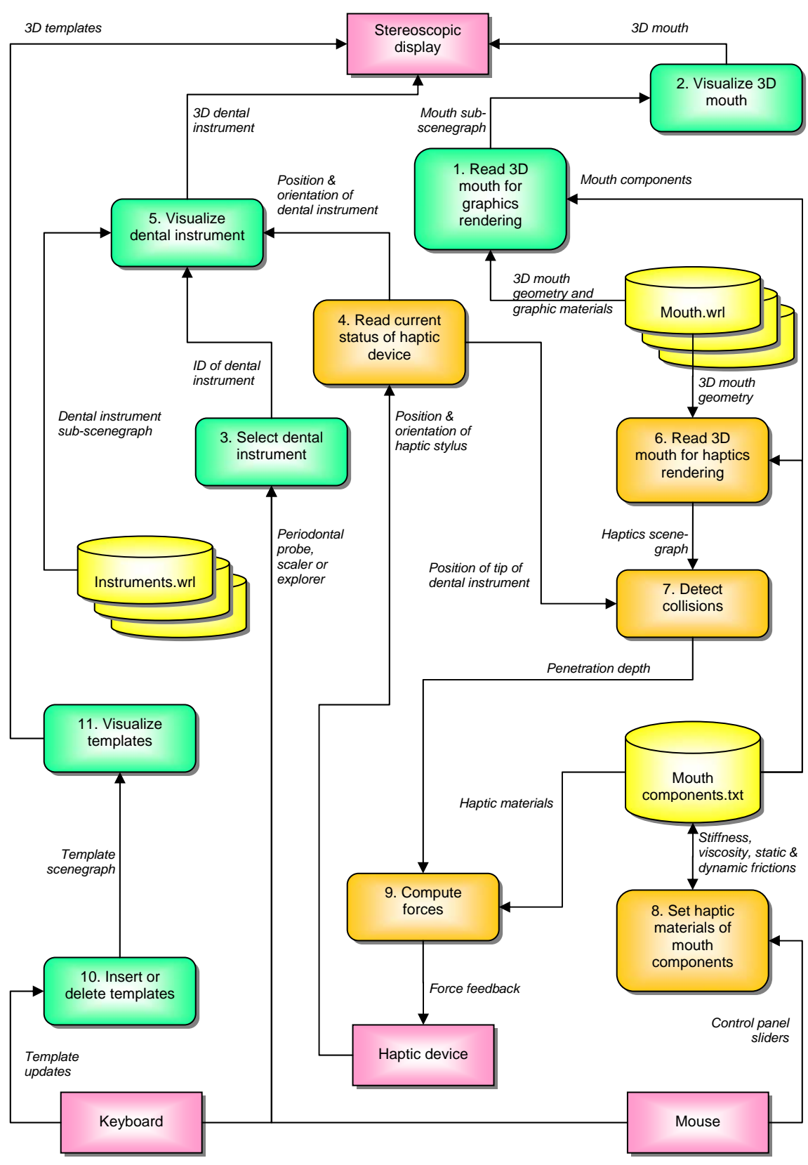
Figure 25. Implementation details of the graphics and haptics rendering processes
