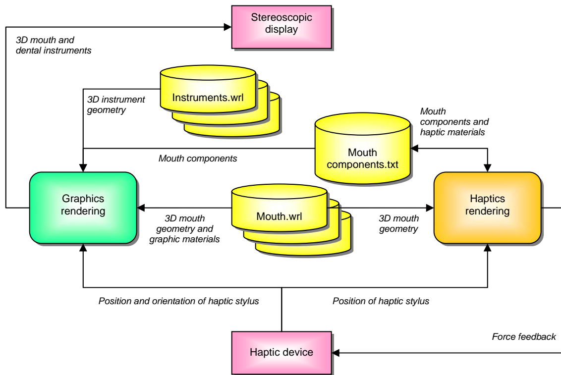
Figure 24. Overview of the implementation of the periodontal simulator
