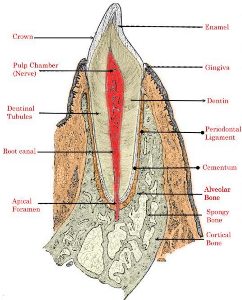
Figure 14. Tooth anatomy [Spiller]
