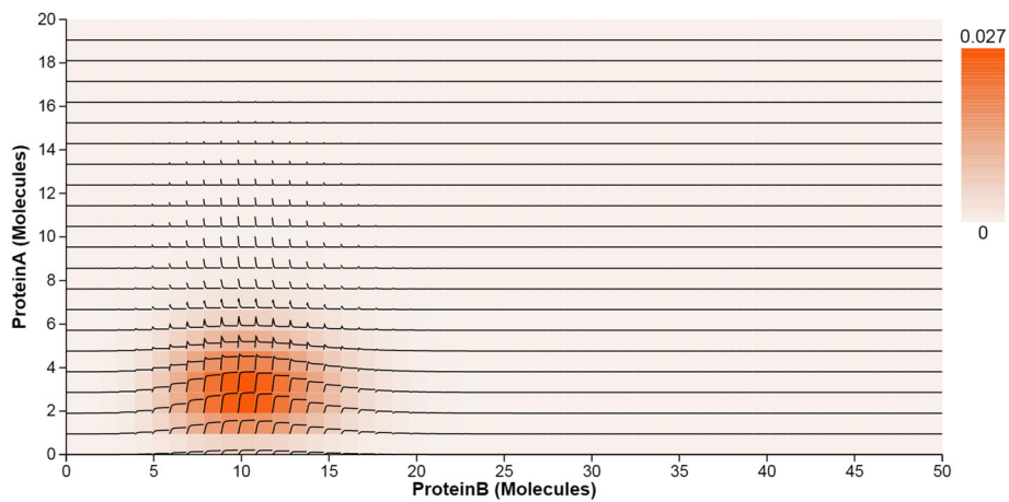
Fig. 4 The 2D heatmap displays the probability distribution over the 2D state space projected for the pair of Pa and Pb. Time Curves overlaid on the 2D heatmap indicate how the probability values in the 2D state space change over time
