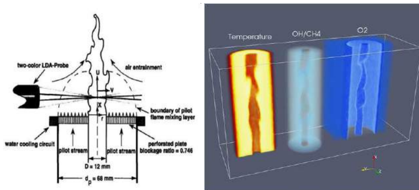
Fig. 1 The experimental setup which introduces the Bunsen burner experiment (left)[4], and example results from a corresponding computational LES model and simulation, showing the gaseous distribution at a specific time-frame (right) [44].
